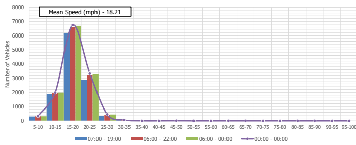
A-B - 5-Day Speed Bin Distributions (mph)
