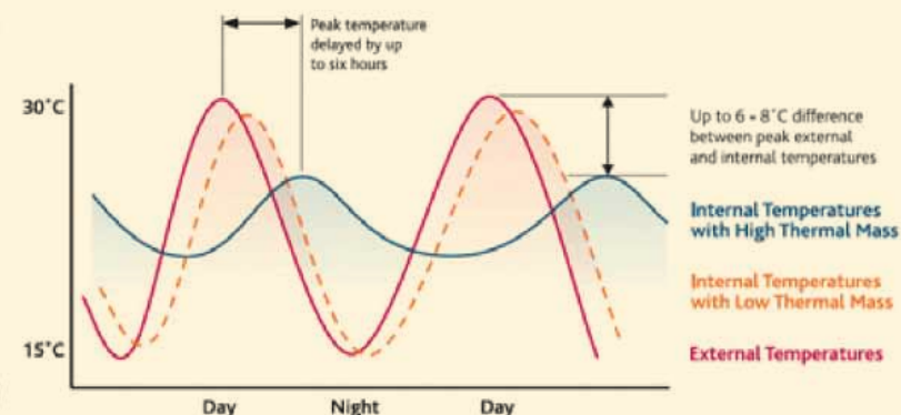
STABILISING EFFECT OF THERMAL MASS ON INTERNAL TEMPERATURE
